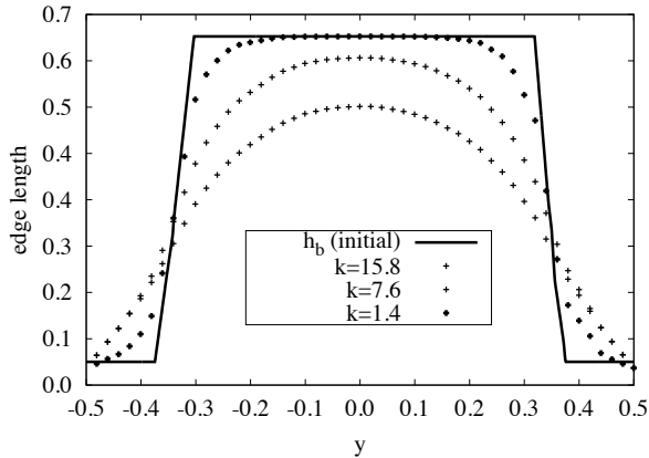
Figure 1: Solutions of the Helmholtz’s equations for different diffusive parameter k
