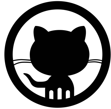
(c) github
